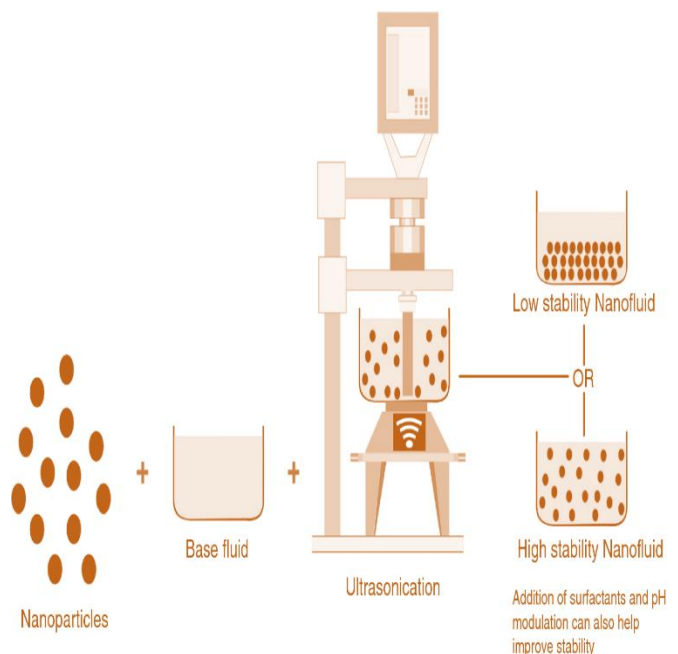
Fig.2. Two-step method of preparing nanofluids [7, 8].
